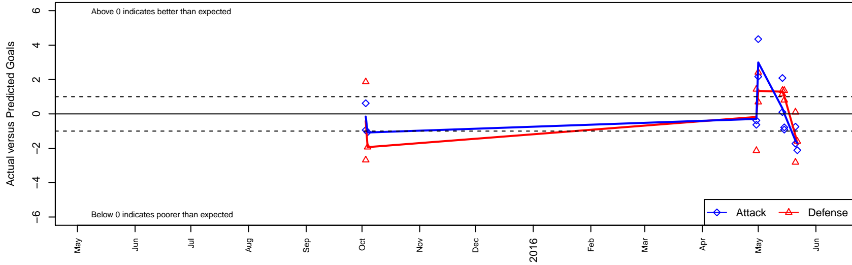
PVSC United Apollo B03 Dots are actual minus expected GF (blue circles) and GA (red triangles). Blue line is smoothed change in attack strength. Red is smoothed change in defense strength.
